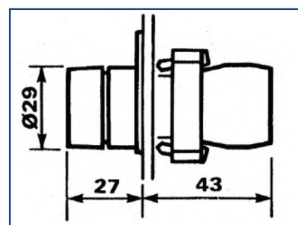
Dimensions:(mm)
