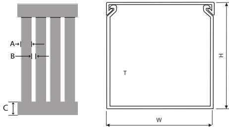
RRE Extrusions-RRX wiring ducts
