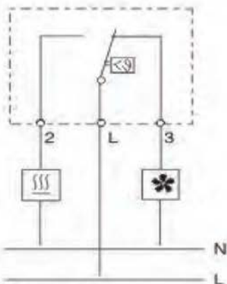
Connection diagram
